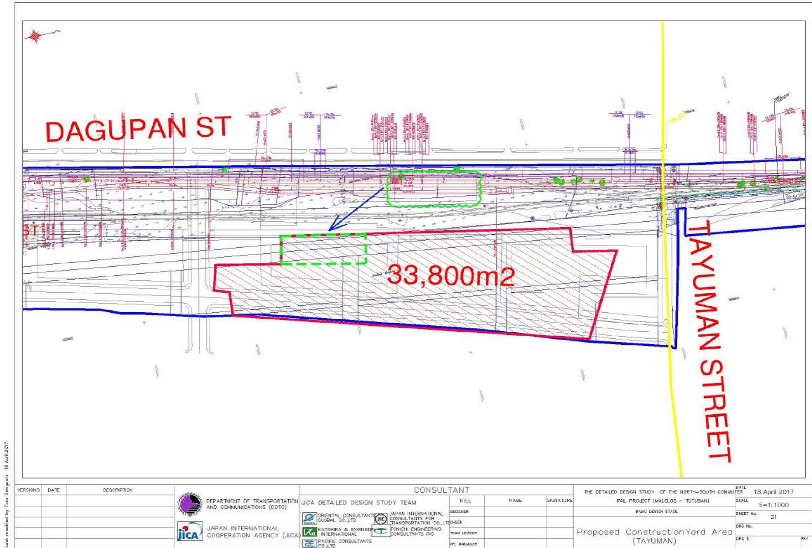
Figure 11.8.5 Construction Yard at Tayuman
