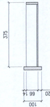
7 SECTION THRU-A 7 SCALE 1 : 25 M
